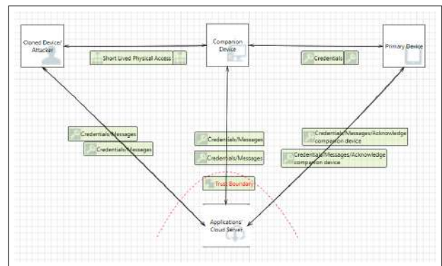
Figure 3: DFD for Signal, WhatsApp, and Telegram desktop applications.
